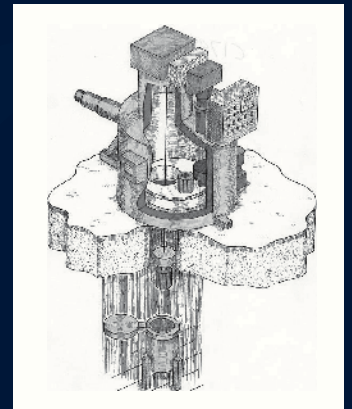
Filter element handling machine Sizewell B
